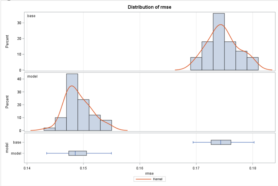
Bootstrapped sampling shows definitive improvement in RMSE ( P < 0.0001 , t=89 , n=50 ) of capital distributions.
