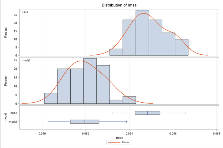
Bootstrapped sampling shows definitive improvement in RMSE ( P < 0.0001 , t=98 , n=50 ) of capital calls.
